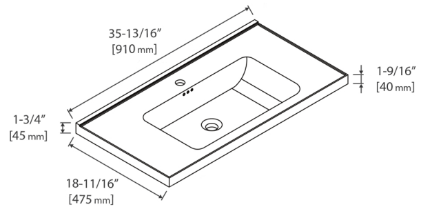
ceramic sink
