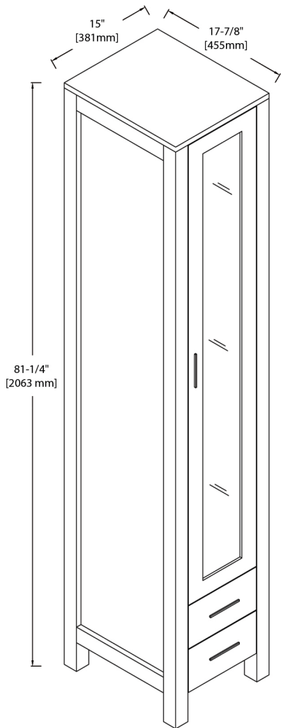
LINEN CABINET FRONT VIEW (V8001 15)
