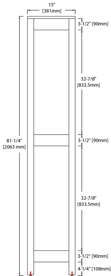
LINEN CABINET BACK VIEW (V8001 15)
