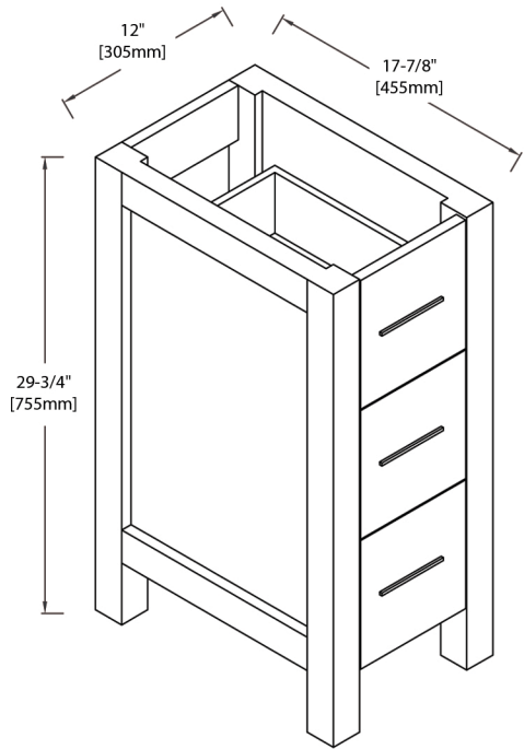
SIDE CABINET FRONT VIEW (S8001 12)
