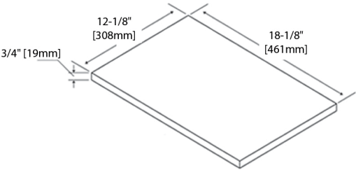
12" SIDE CABINET COUNTERTOP (CT5001 1218 01)
