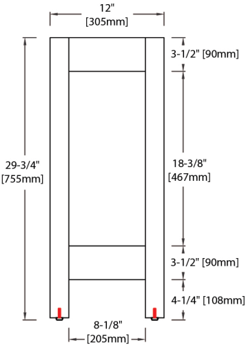
SIDE CABINET BACK VIEW (S8001 12)
