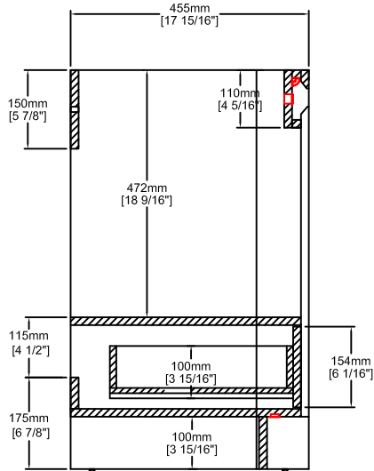
SECTION VIEW
